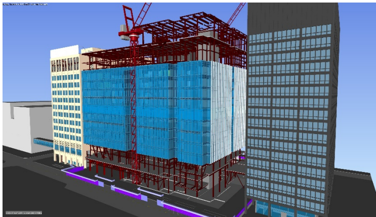
Exterior Wall Cladding December 2017
